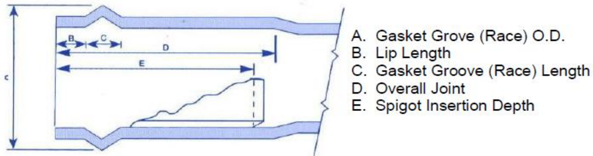
LOCKED-IN GASKET JOINT
