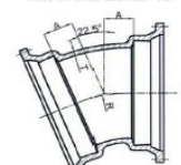
MJ x MJ Bend 22-1/2
