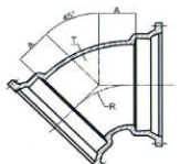
MJ x MJ Bend 45
