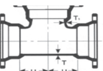
MJ x MJ DMT
